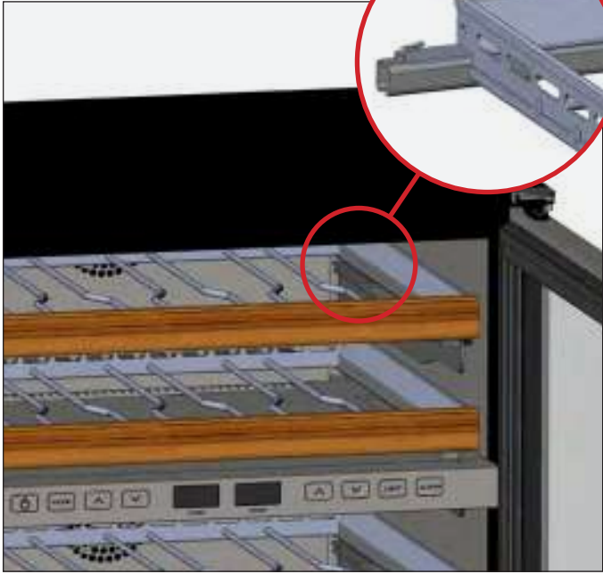
FIG. 4. Be sure the wine rack sits under the rear tabs.
