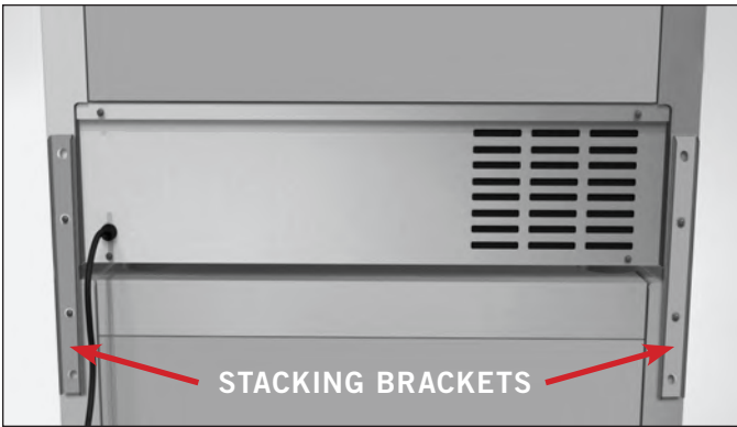
FIG. 1. The rear stacking brackets.
