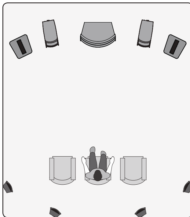
MartinLogan electrostatic speakers as front channels, center channel, and rear and side surround (effects) channels. MartinLogan subwoofers as LFE (effects) channel.
