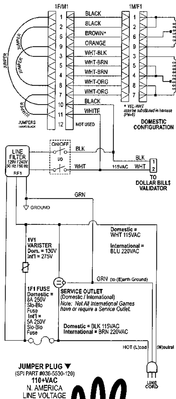
Transformer Power Wiring Diagram
