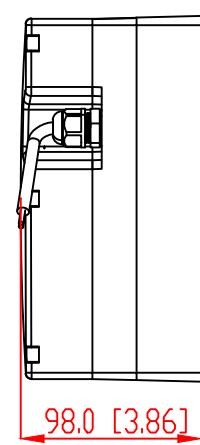
MOUNTING DEPTH
