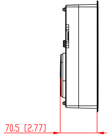
MOUNTING DEPTH
