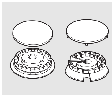
Surface Burner Heads & Caps
