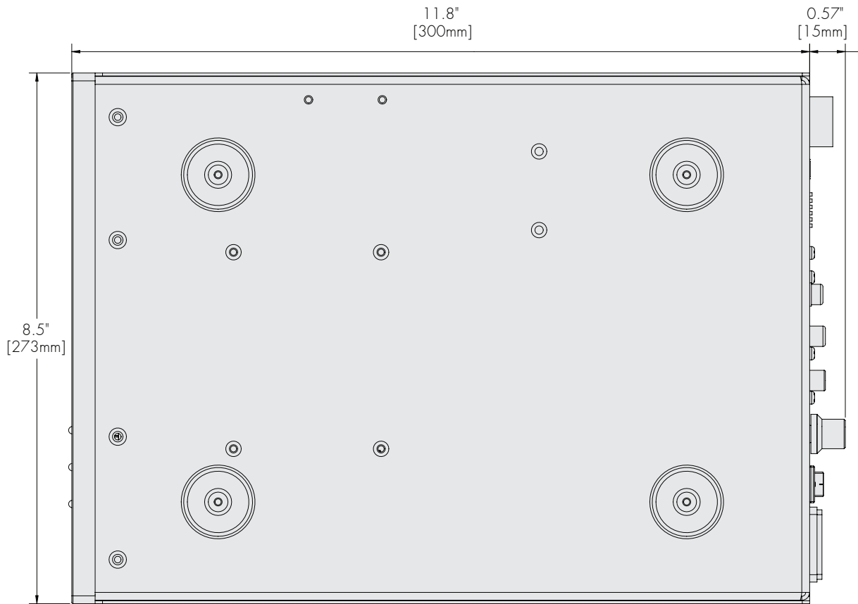
BOTTOM VIEW
