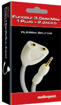
FLX-Mini Splitter 3.5mm Mini Male Stereo > (2) 3.5mm Female Stereo Metal: Solid Perfect-Surface Copper+ (PSC+) Length: 15cm (6 in.) Retail: 22.95
