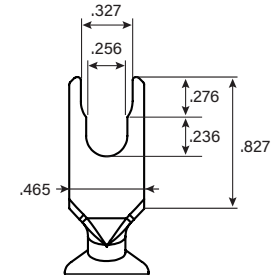
Multi-Spade Dimensions (in.)
