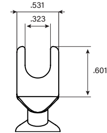
U-Spade Dimensions (in.)
