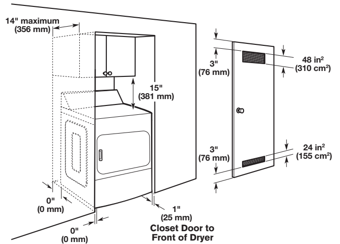
Side View, Recessed In Closet
