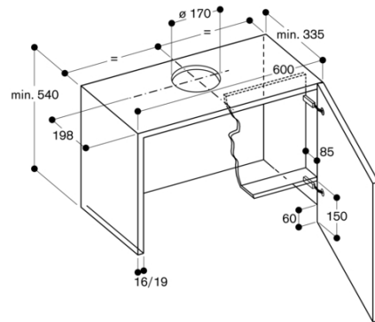
Top cabinet for AF 200 160 with lowering frame AA 210 460
