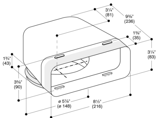
Measurements in inches (mm)
