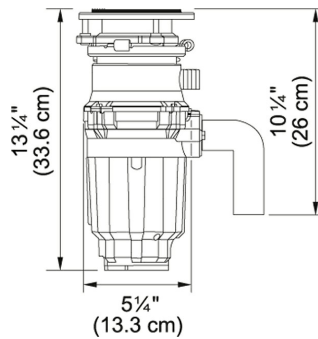
Technical Drawing
