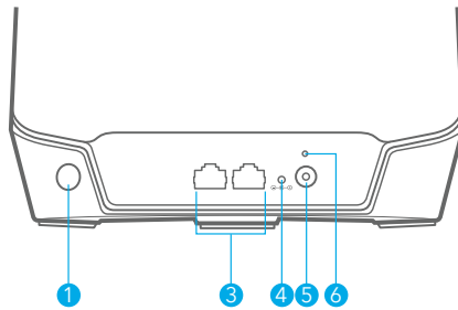
Orbi Satellite
