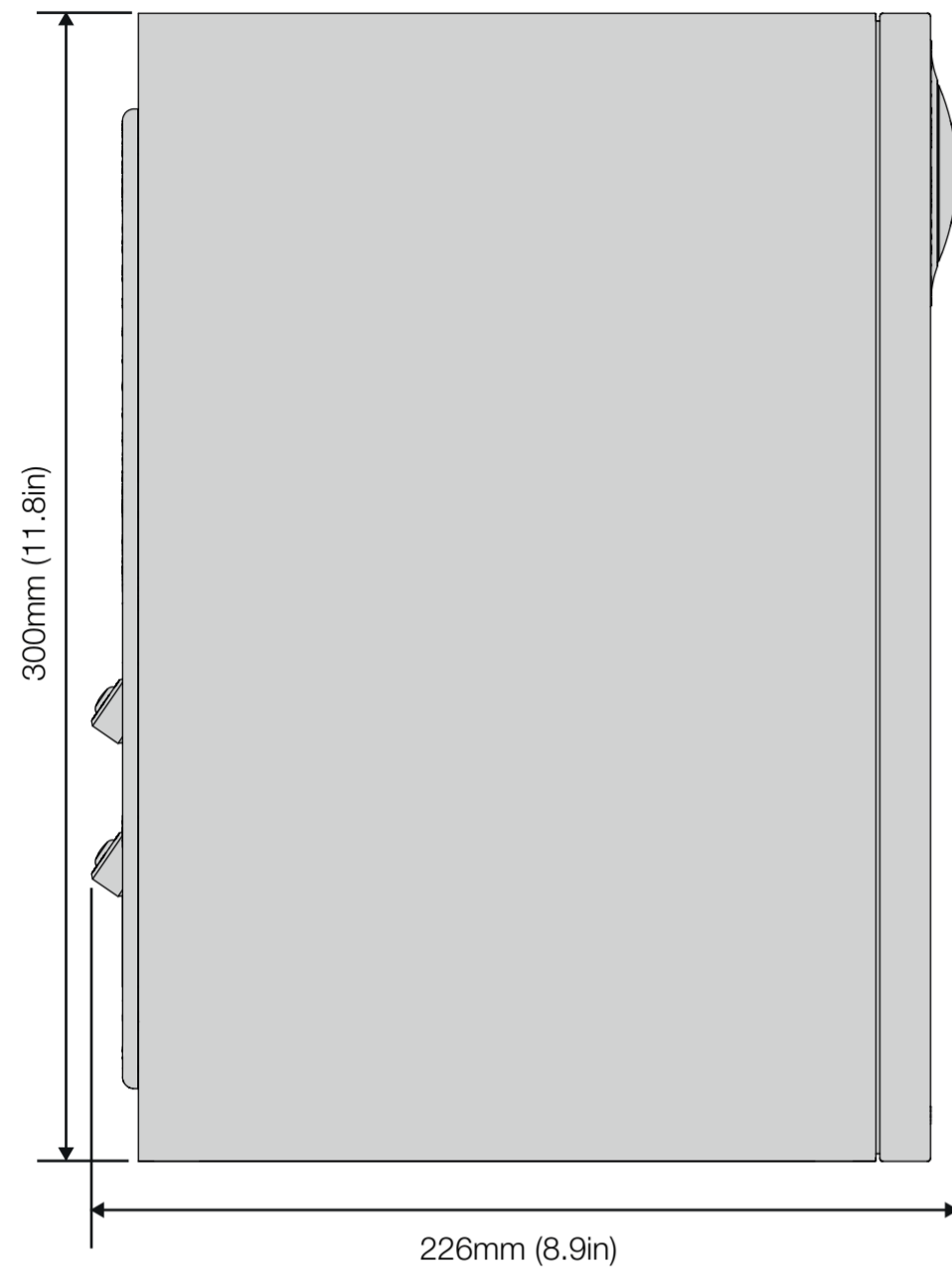
SIDE
