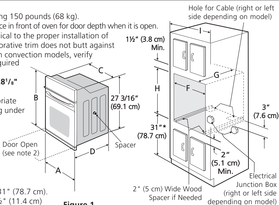
Figure 1 27" and 30" Single Wall Ovens (Double ovens see Figure 2)
